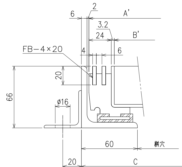
断面詳細 (S=1/2)
