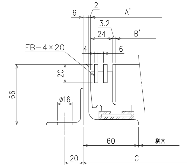
断面詳細 (S=1/2)
