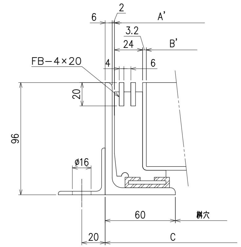
断面詳細 (S=1/2)
